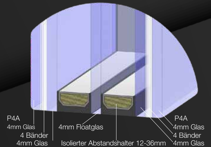
P4A+4mm Floatglas+P4A
